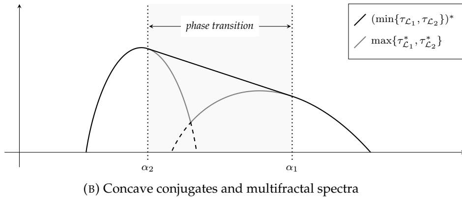
FIGURE 2. An example illustrating a non-trivial phase transition
